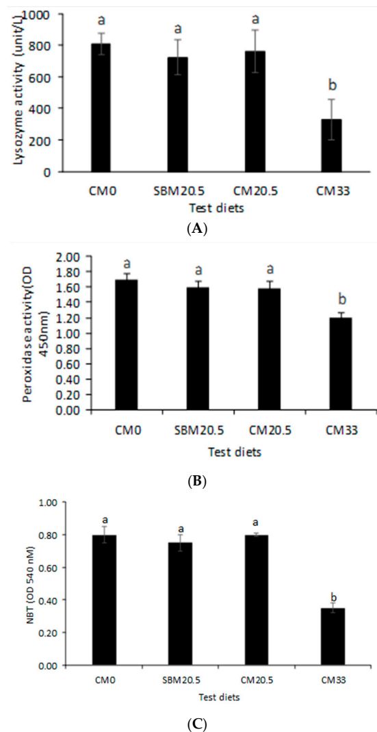
Figure 1. (A) Serum lysozyme activity (U/L, n = 3 ); (B); serum peroxidase activity ( n = 3 ); (C) nitro blue tetrazolium (%; mean ± standard error, n = 3 ) of nutrients in red seabream fed diets formulated by replacing fish meal with camelina meal at 0% for reference diet (CM0), 20.5 g/kg with soybean meal (SBM20.5), 20.5 g/kg with camelina meal (CM20.5) and 33 g/kg camelina meal (CM33). Values with different letters are significantly different ( p < 0.05 ).
